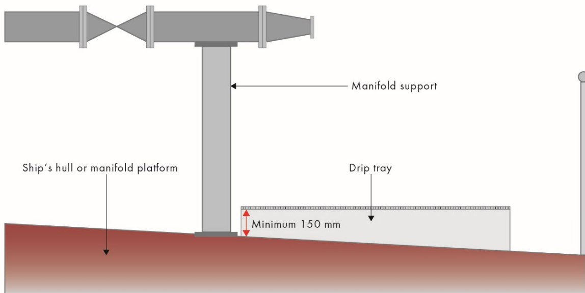
Figure Ad1: Minimum depth of manifold drip tray
